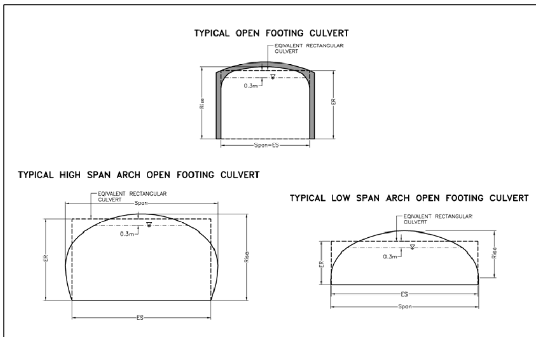
Figure WC7.1 – Clearance for Non-Rectangular Culverts
